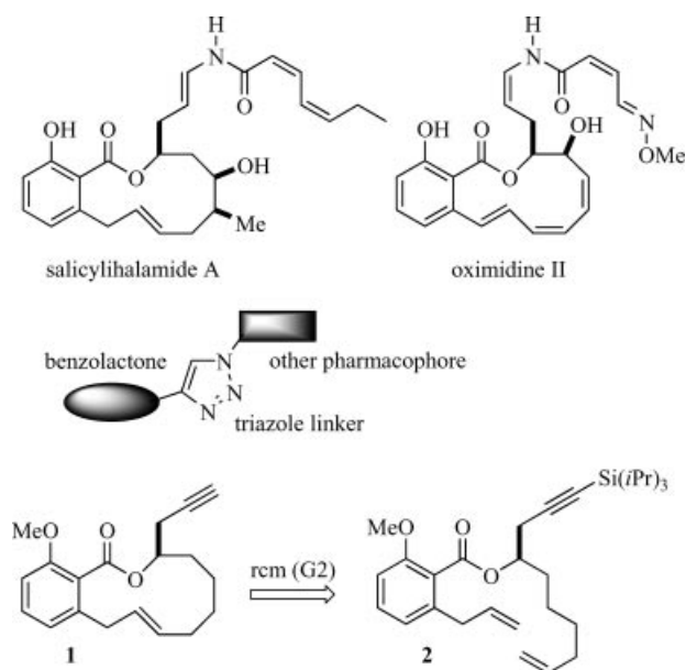
Figure 3. Design of dual domain benzolactone analogs utilizing click chemistry on alkyne 1 .
