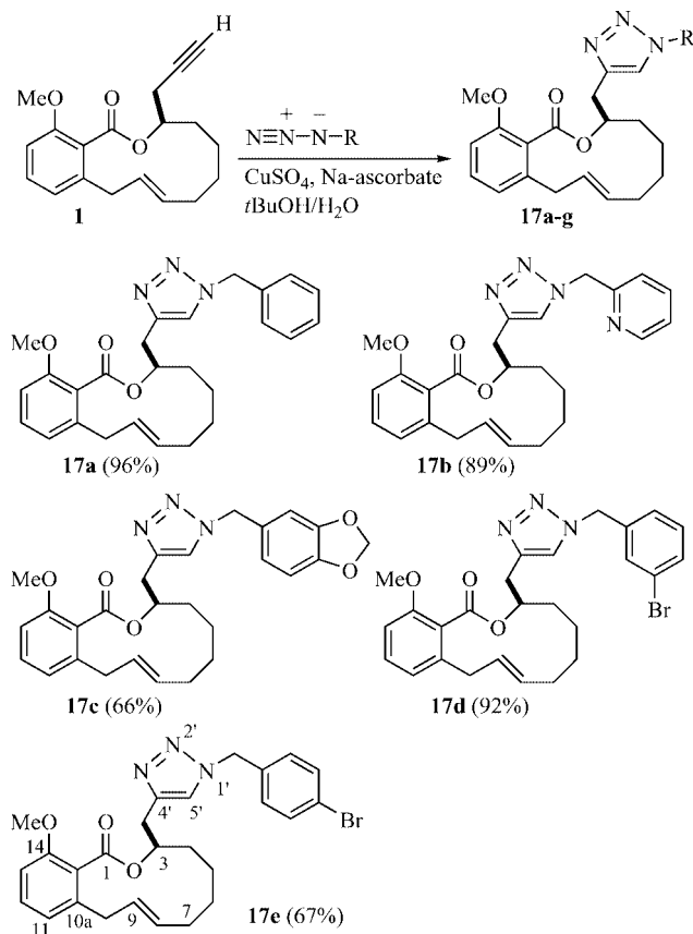
Scheme 4. Synthesis of the triazoles 17a–e using the corresponding benzylic azides and lactone 1 .
