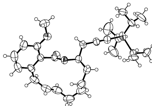
Figure 4. X-ray structure of macrolactone E-12 .
