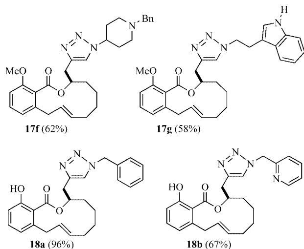
Scheme 5. Synthesis of the triazoles 17f and 17g from lactone 1 . Cleavage of the aromatic methyl ether to give the lactone-triazole conjugates 18a and 18b .
