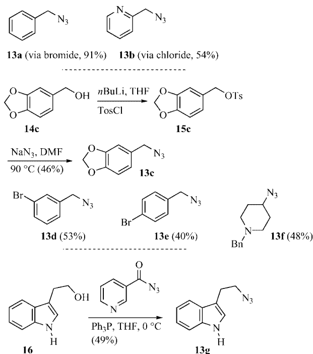
Scheme 3. Synthesis of the azides 13a–g by S N 2 reactions.
