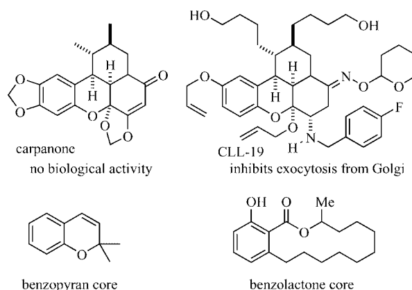
Figure 1. A natural product library based on carpanone and two privileged core structures.
