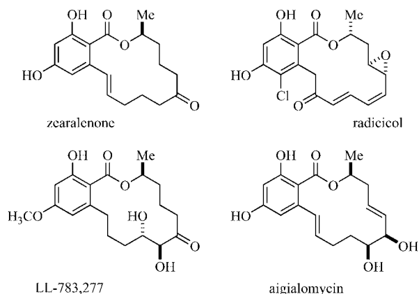
Figure 2. Typical 14-membered benzolactones with a methyl substituent.
