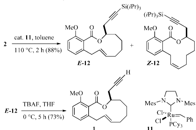
Scheme 2. Ring-closing metathesis of benzoate 2 using Grubbs catalyst II ( 11 ).
