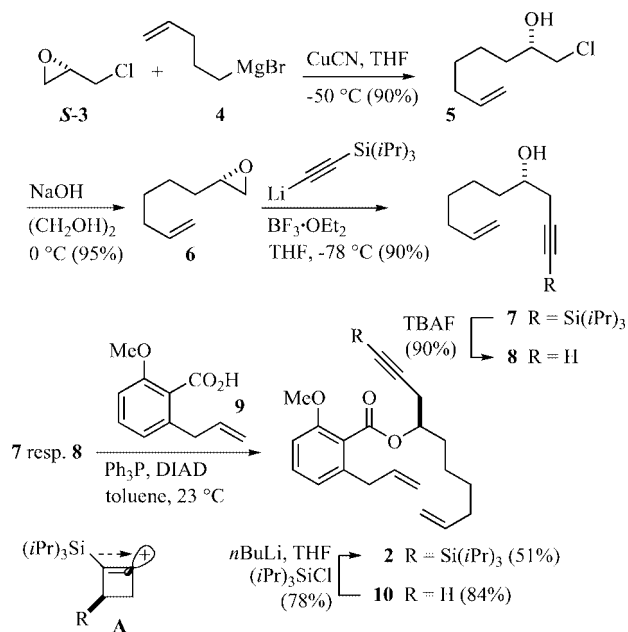
Scheme 1. Synthesis of the benzoate 2 via Mitsunobu esterification of acid 9 with alkynol 7 .
